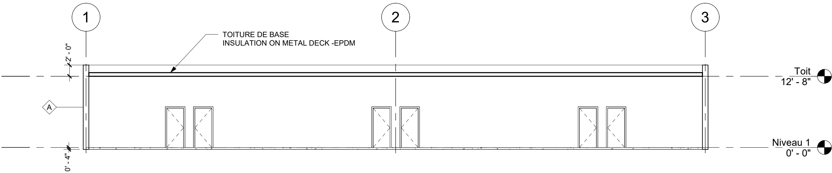
A Coupe A 1" = 10'-0"
